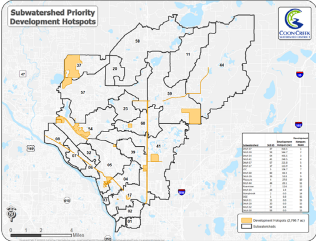
Figure 1.40. Active and anticipated development hotspots in the watershed
