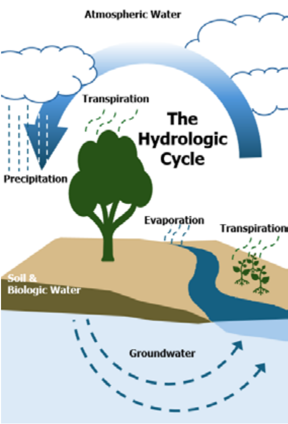
Figure 3.10. Hydrologic water cycle
