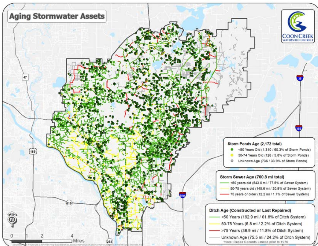
Figure 3.27. Stormwater assets in the CCWD
