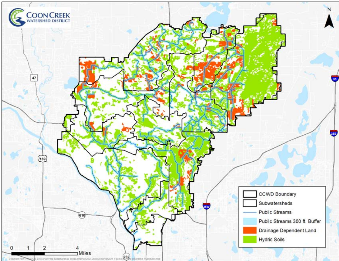
Figure 3.08. District drainage system summary
