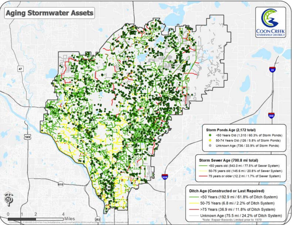
Figure 3.06. Stormwater asset inventory
