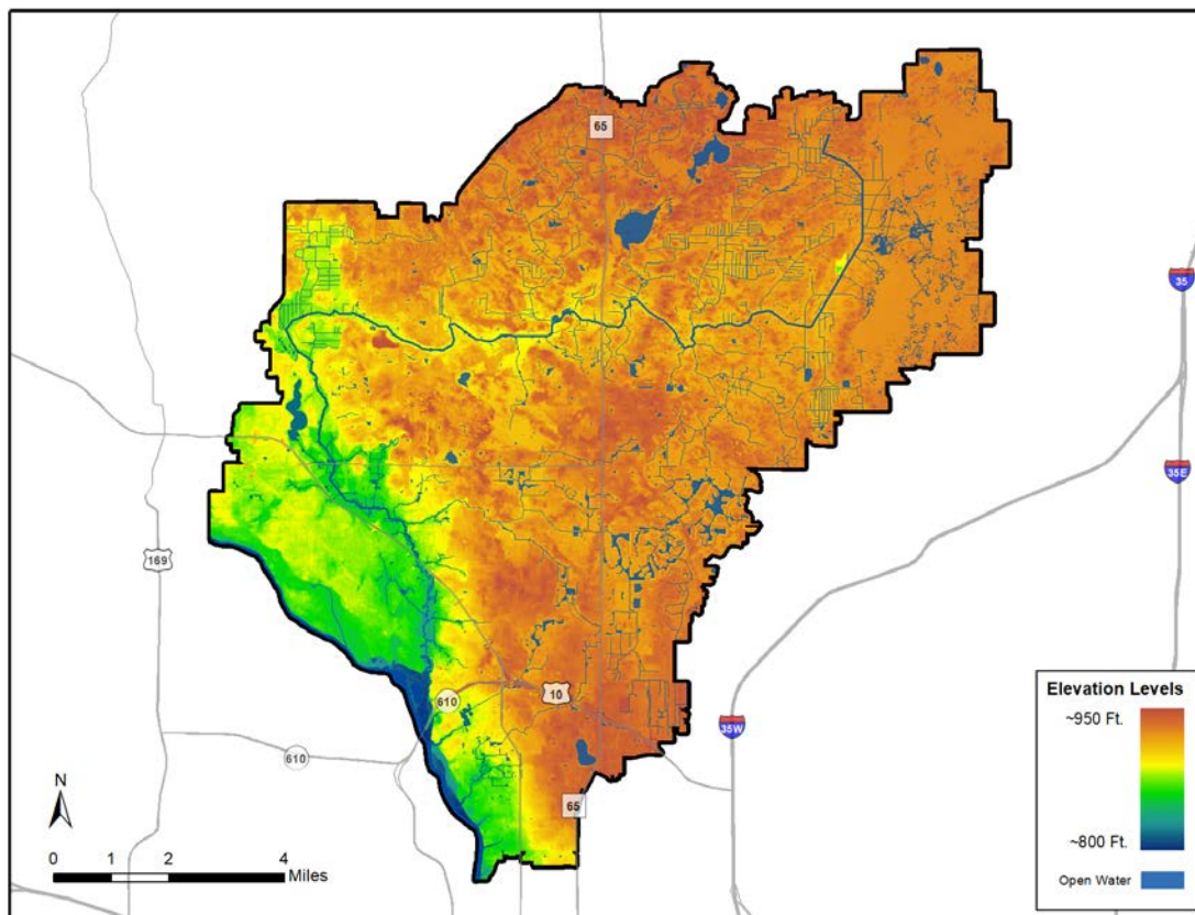
Figure 3.41. CCWD topography
