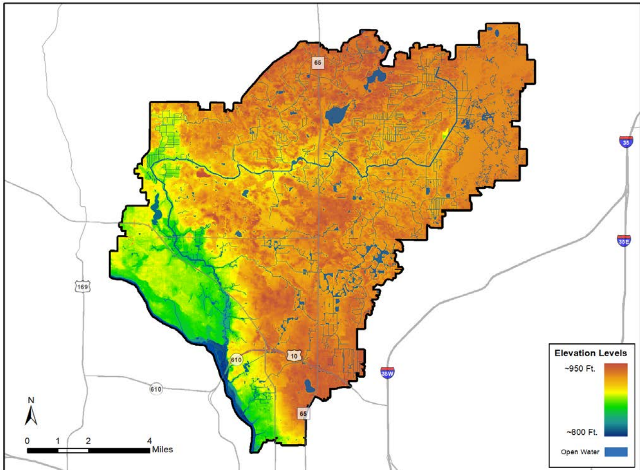
Figure 3.13. CCWD topography
