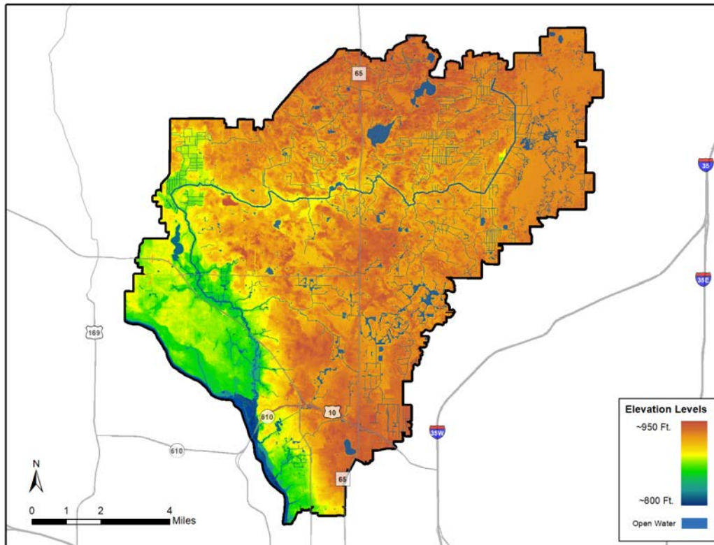
Figure 3.02. CCWD topography
