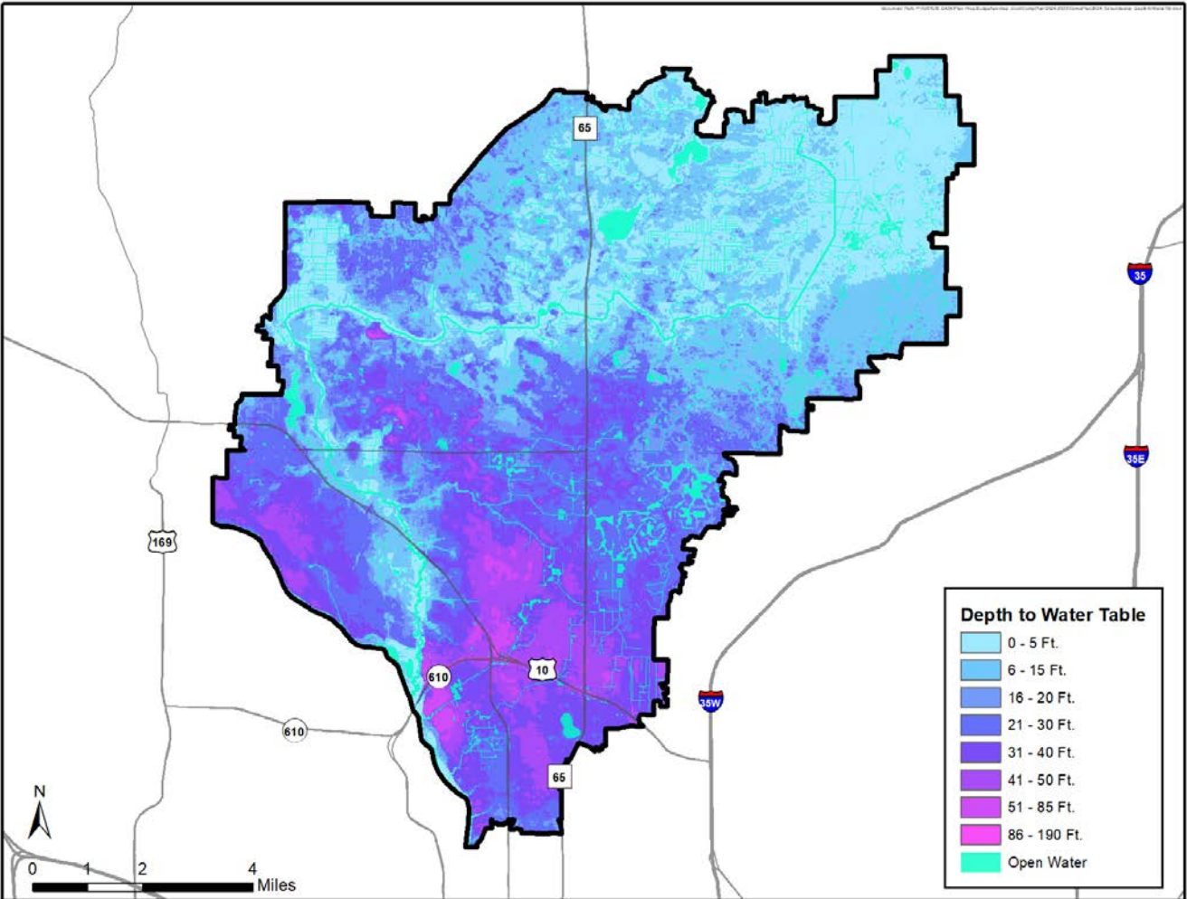
Figure 3.14. District hydrology
