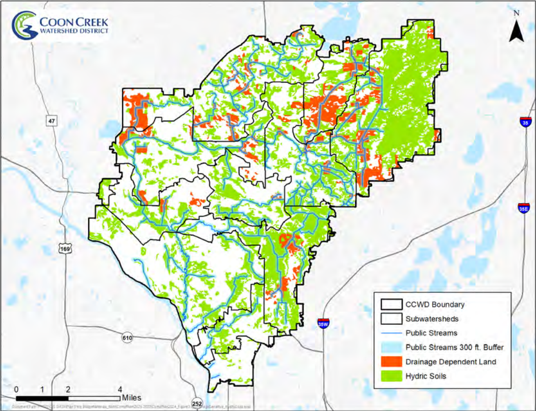
Figure 3.08. District drainage system summary
