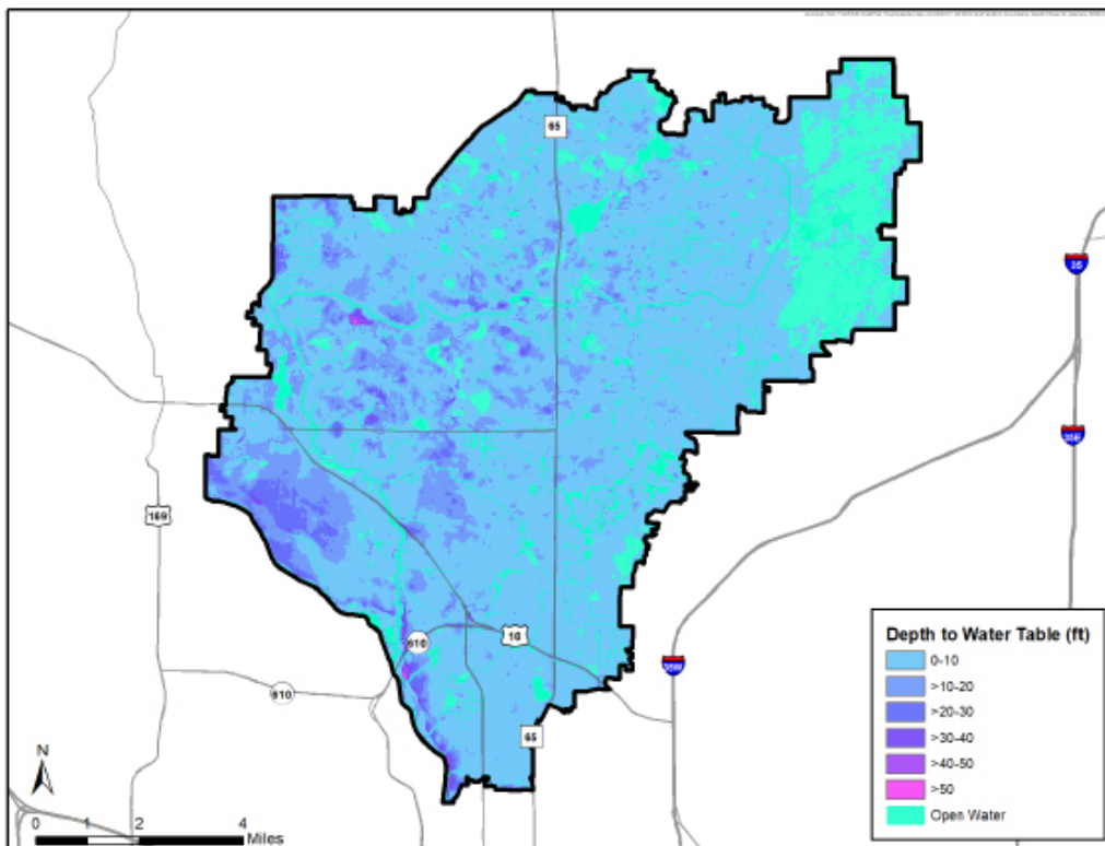
Figure 3.03. Depth to water table in the watershed
