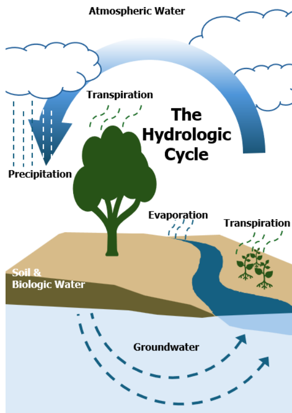
Figure 3.10. Hydrologic water cycle
